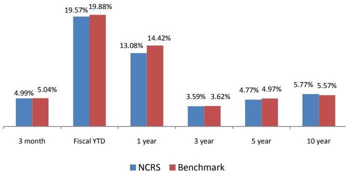
Portfolio Return (NCRS) vs. Benchmark
