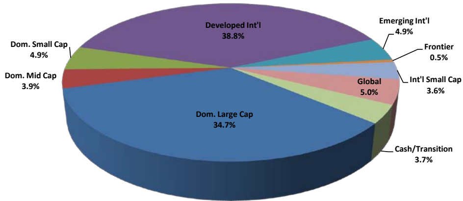
Fund Allocation (based on fund mandate)
